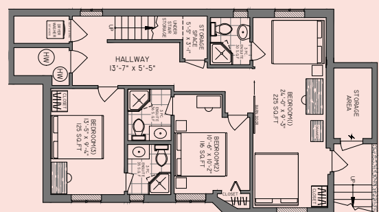
LOWER FLOOR
